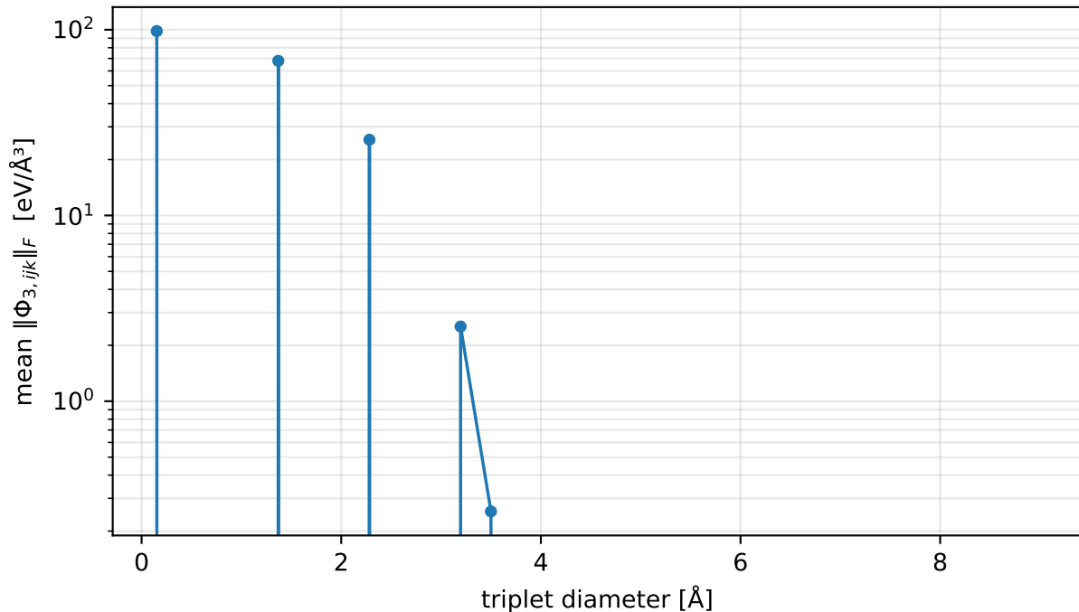
FC3 magnitude vs triplet diameter — sinw100_d5a_vasp
