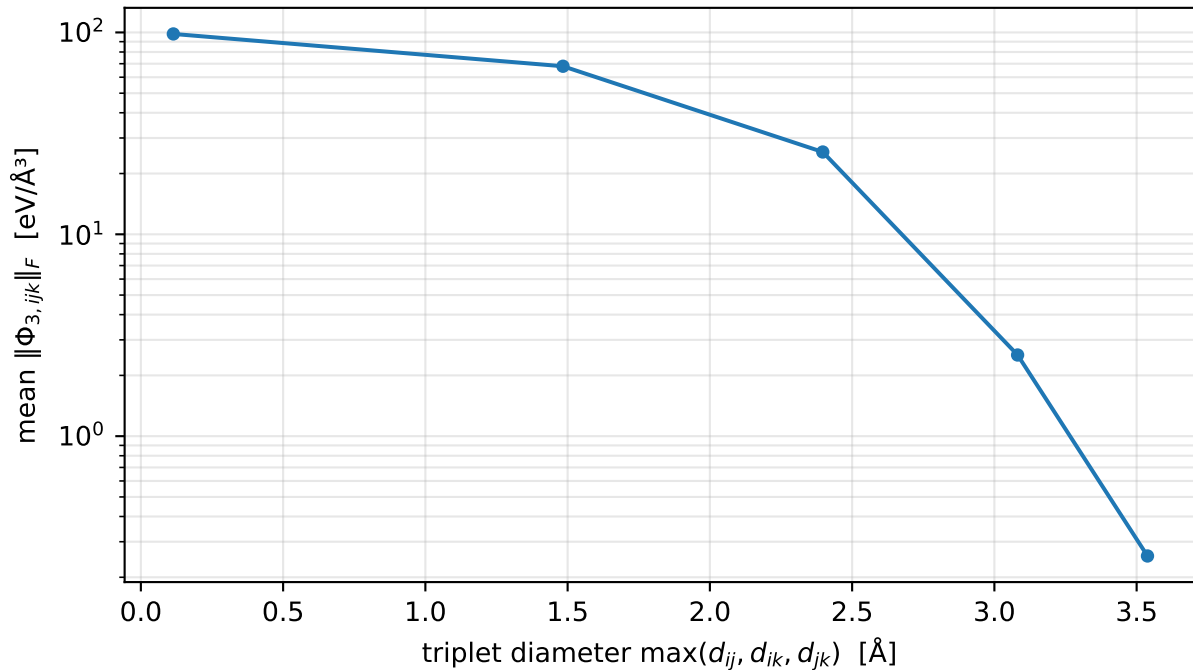
FC3 magnitude decay vs. triplet diameter — sinw100_d5a_vasp
