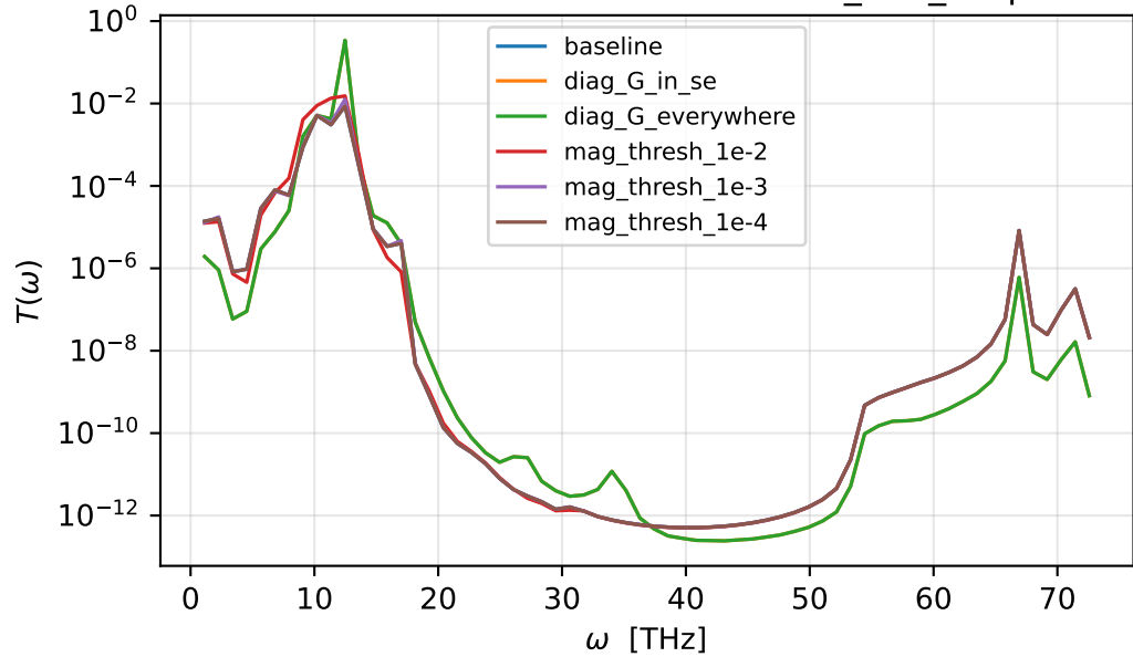
Ballistic transmission — sinw100_d5a_vasp
