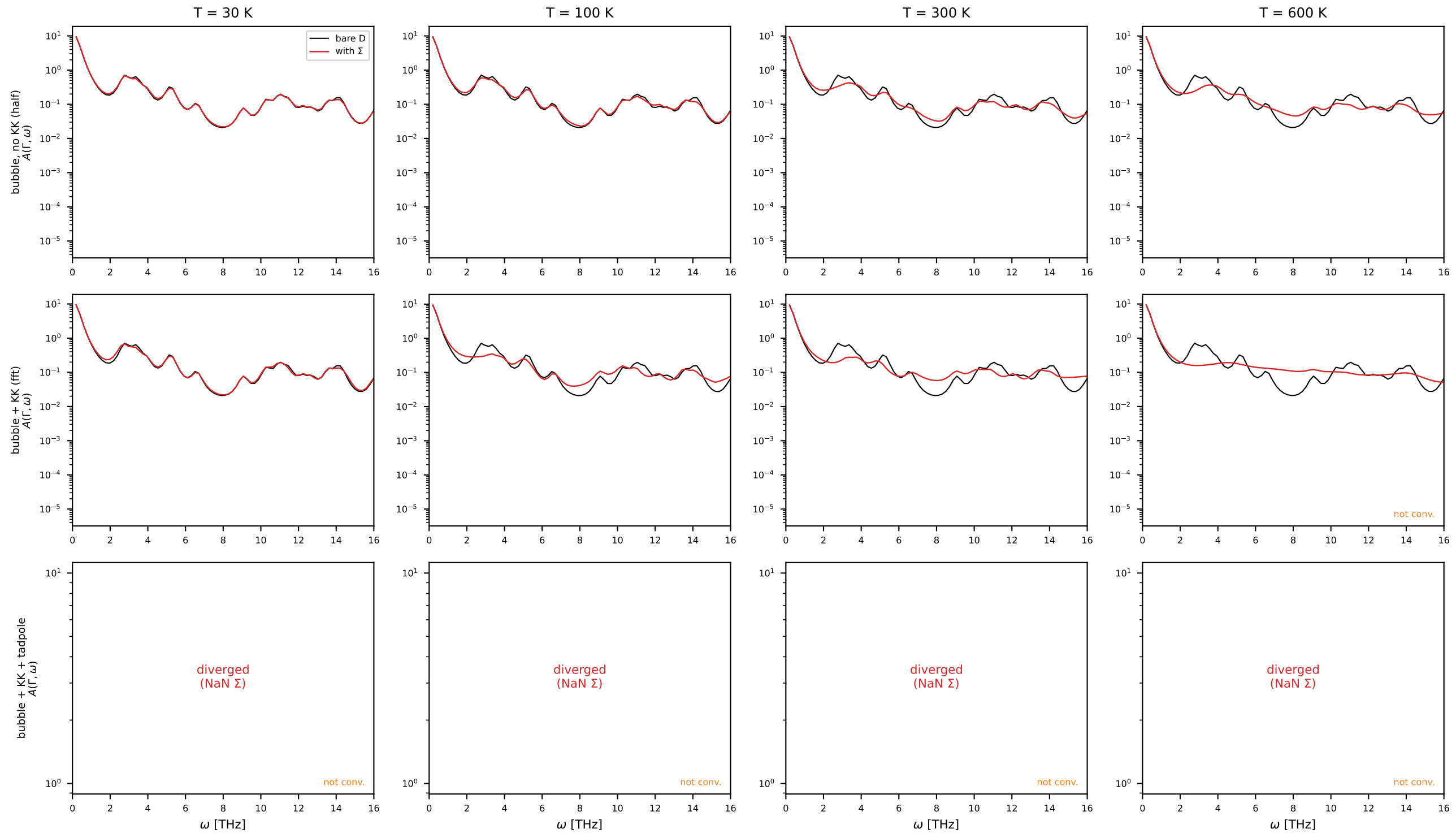
d5a: spectral function with vs without self-energy
