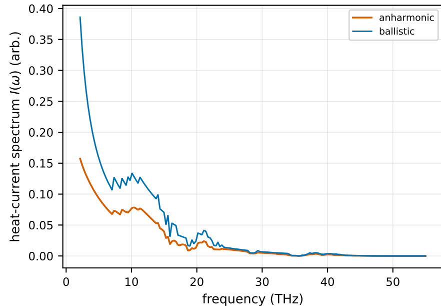
cnt33 \eta = 0 : 3-phonon suppression
