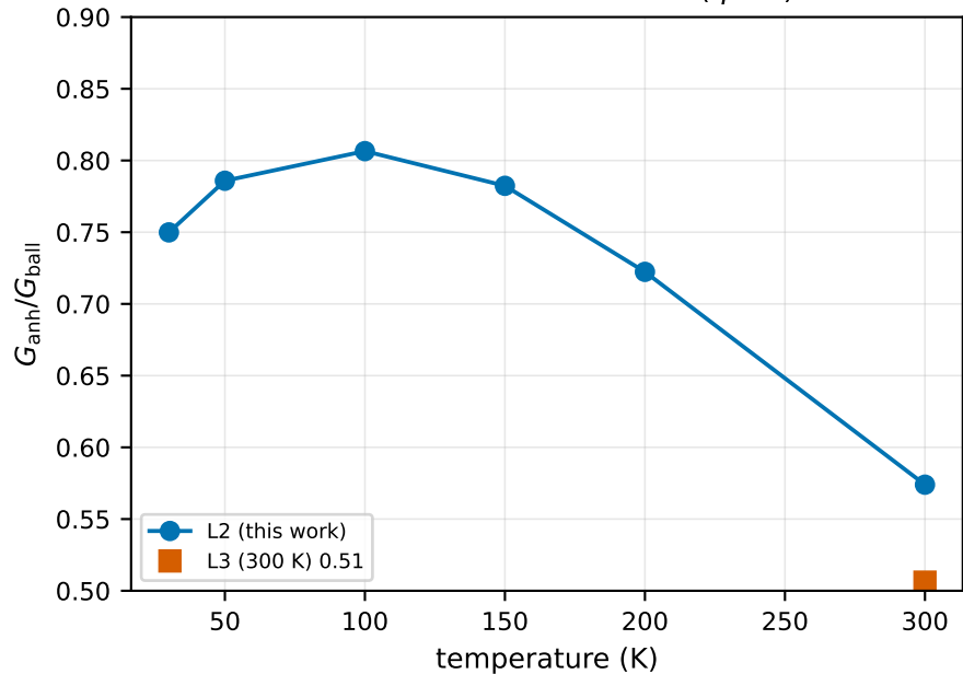
anharmonic reduction vs T ( \eta = 0 )
