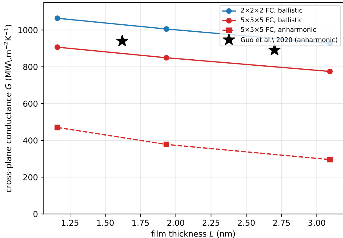
Si thin film, cross-plane conductance vs. \ Guo 2020
