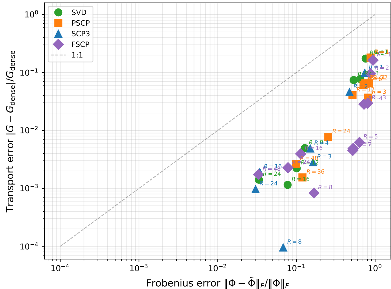
Frobenius vs transport error
