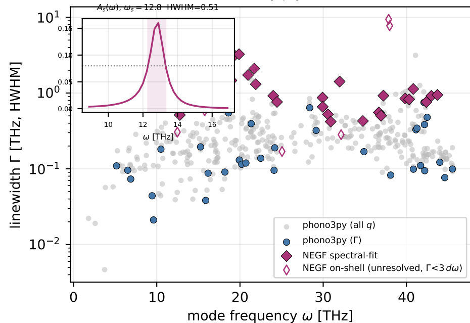
CNT(3,3)
