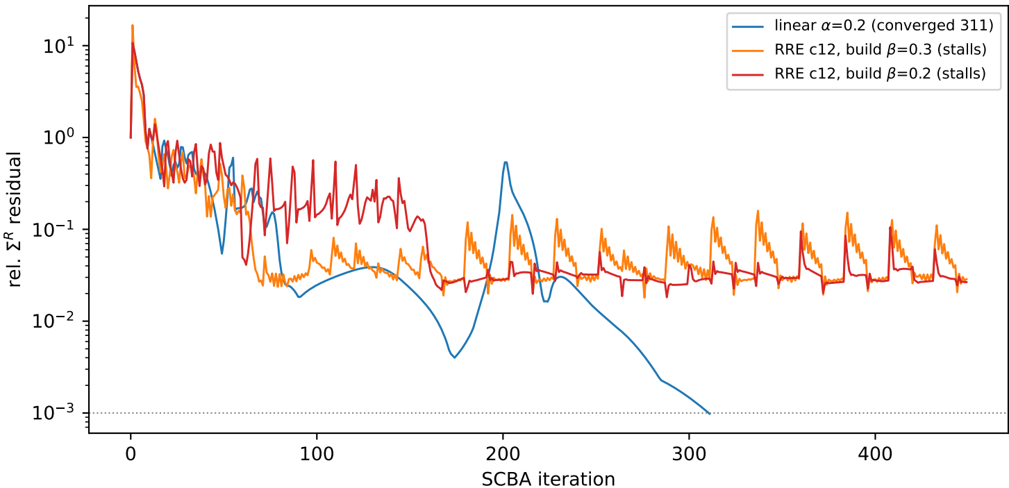
L4, exact kernel: plain linear still beats RRE
