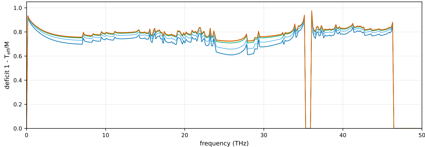
spectral transmission deficit
