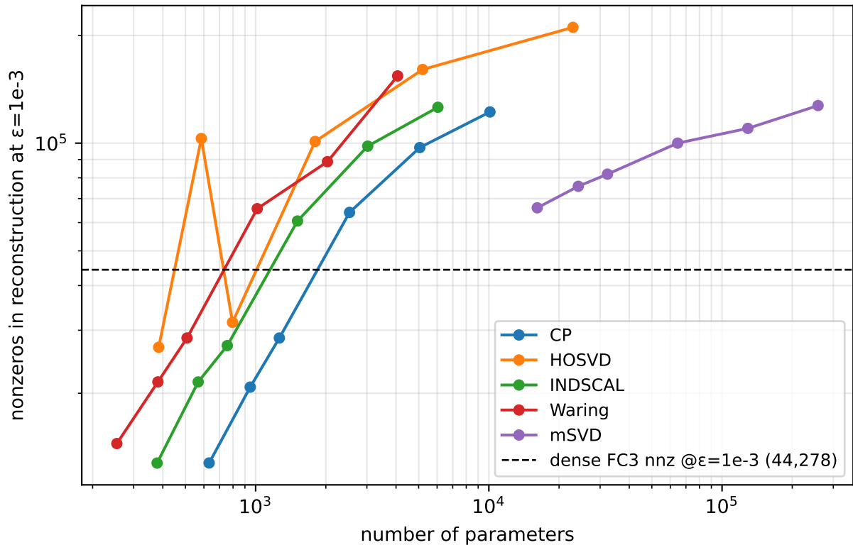
FC3 decomposition: reconstruction nnz vs. parameter count — sinw100_d5a
