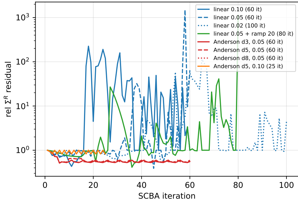
cnt33 L2, conserving vertex, \eta=0.45 , 121 pts
