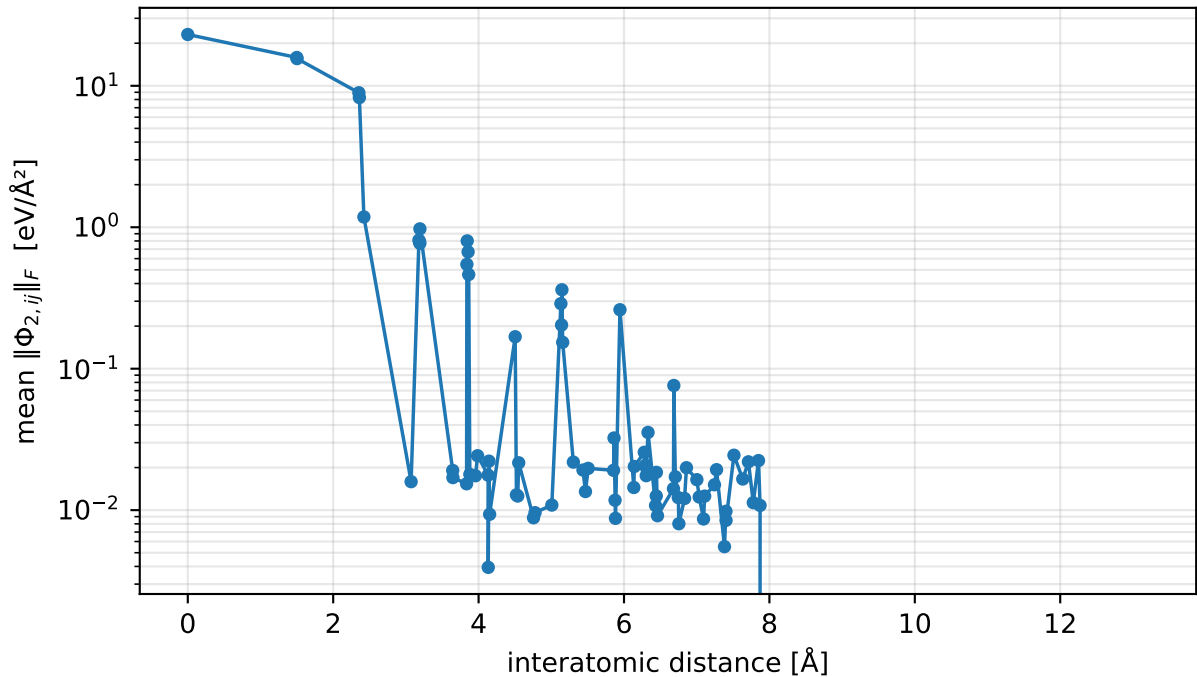
FC2 magnitude vs distance — sinw100_d5a_vasp_sc4
