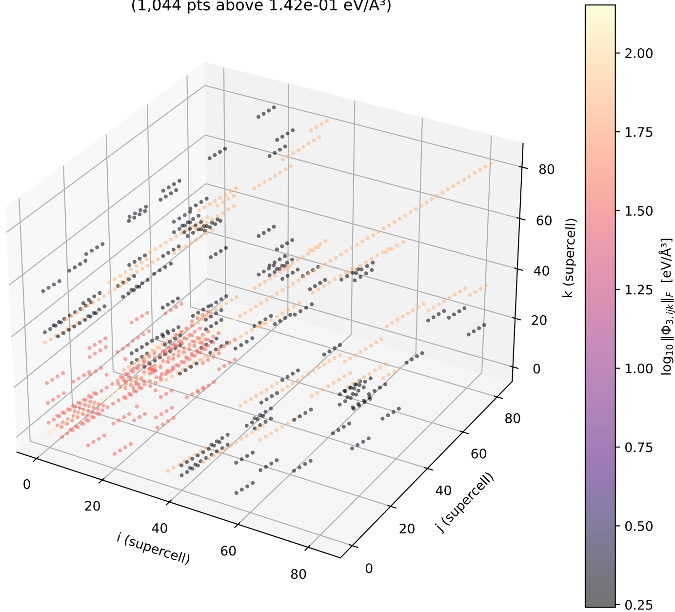
FC3 support — sinw100_d5a_vasp_sc4 (1,044 pts above 1.42e-01 eV/Å 3 )
