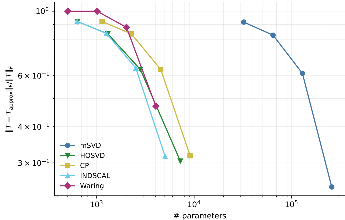
FC3 approximation quality — Frobenius residual
