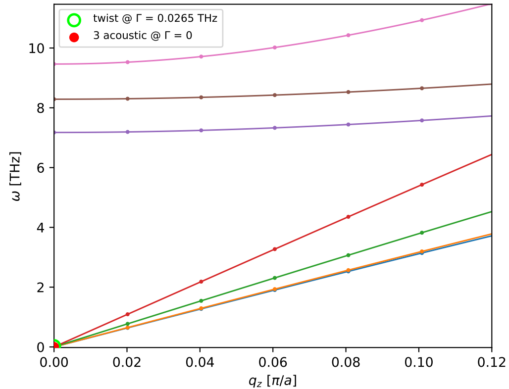
CNT(3,3): branches near \Gamma
