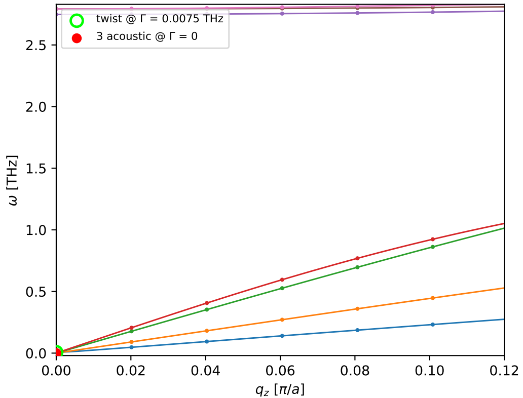
SiNW d5a: branches near \Gamma
