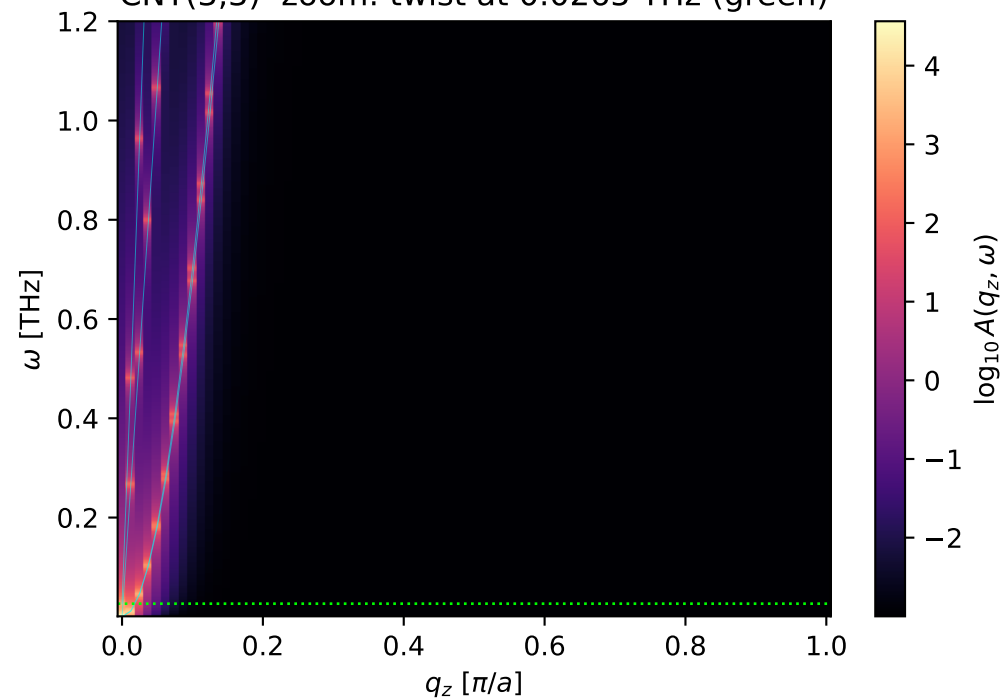
CNT(3,3) zoom: twist at 0.0265 THz (green)
