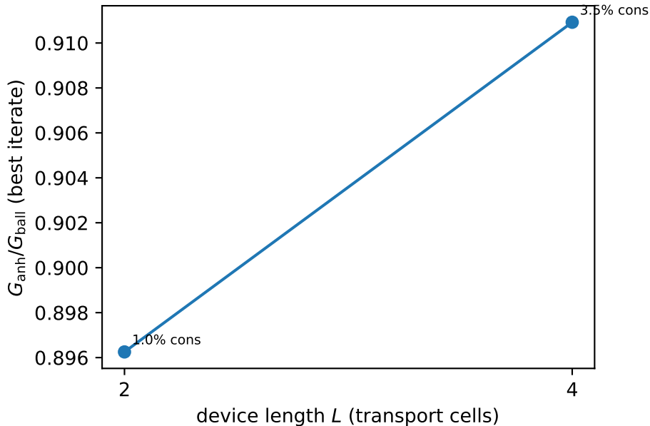
Production CNT(3,3) length ladder ( \eta=0.45 )
