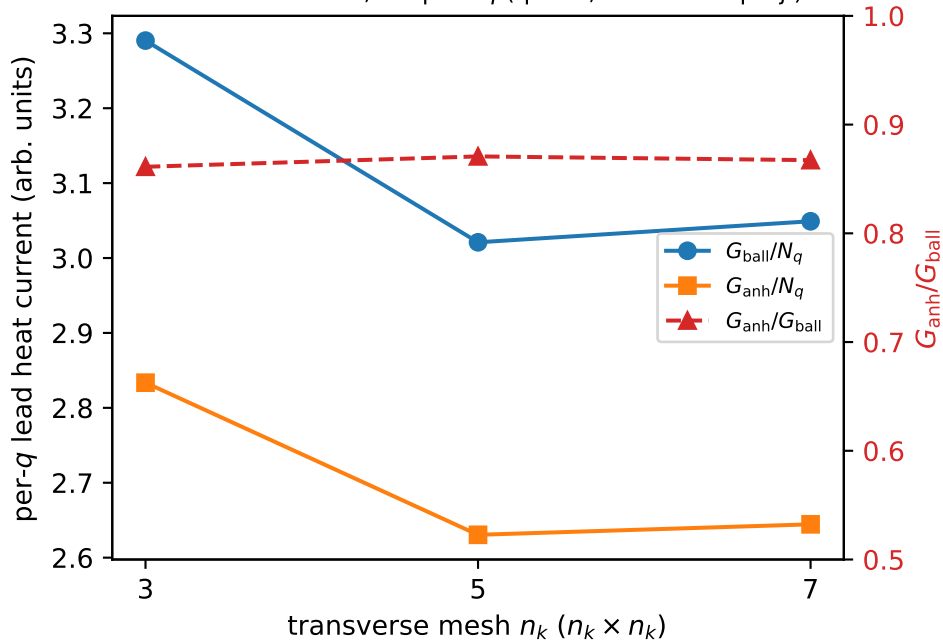
Production Si film, coupled- q ( \eta=0.4 , zero-mode proj.)
