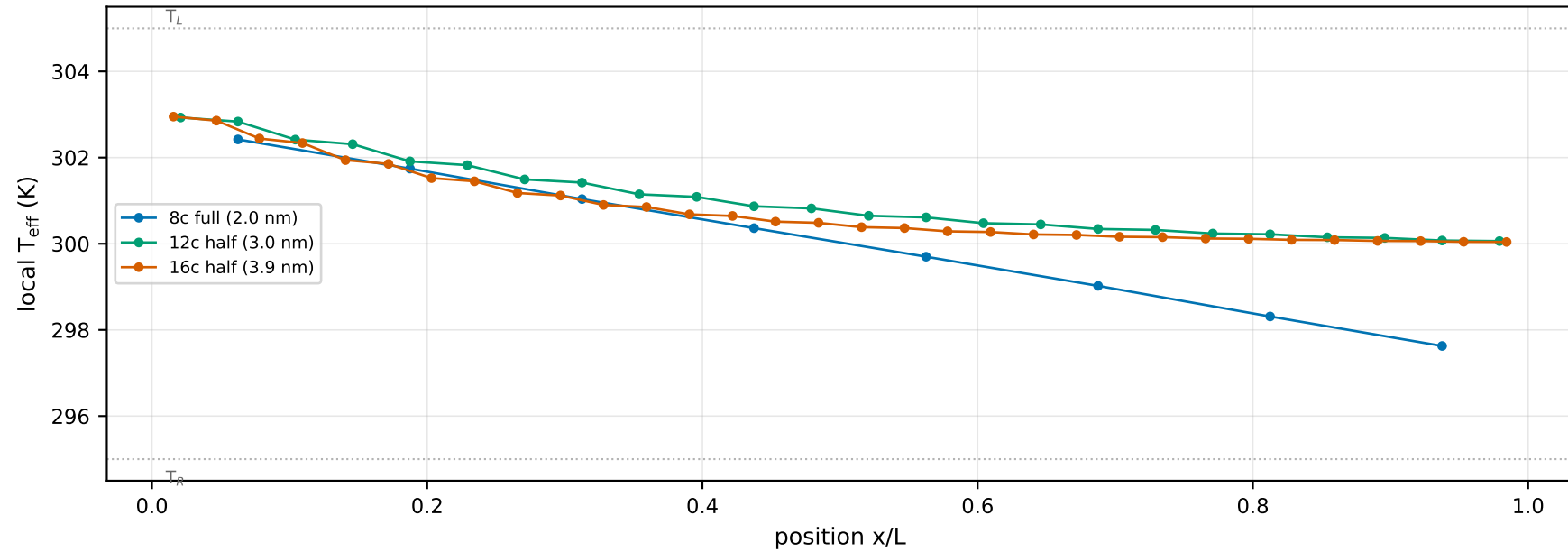
slab-resolved effective temperature
