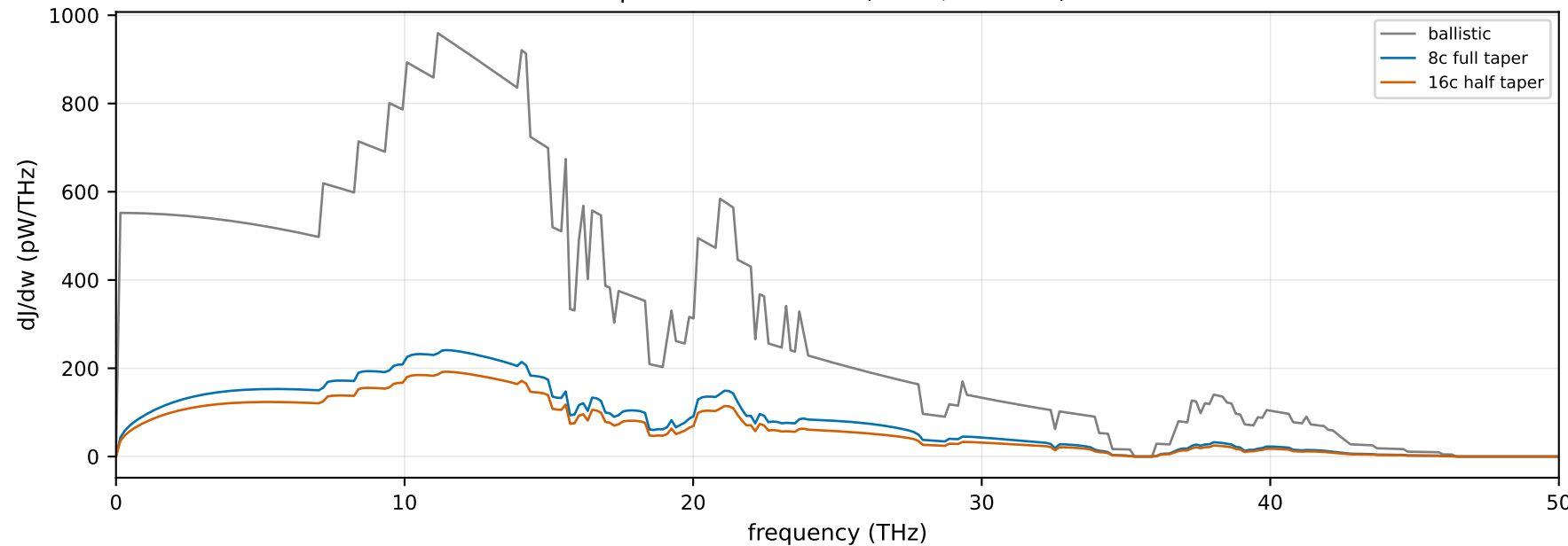
spectral heat current (300 K, dT=10 K)
