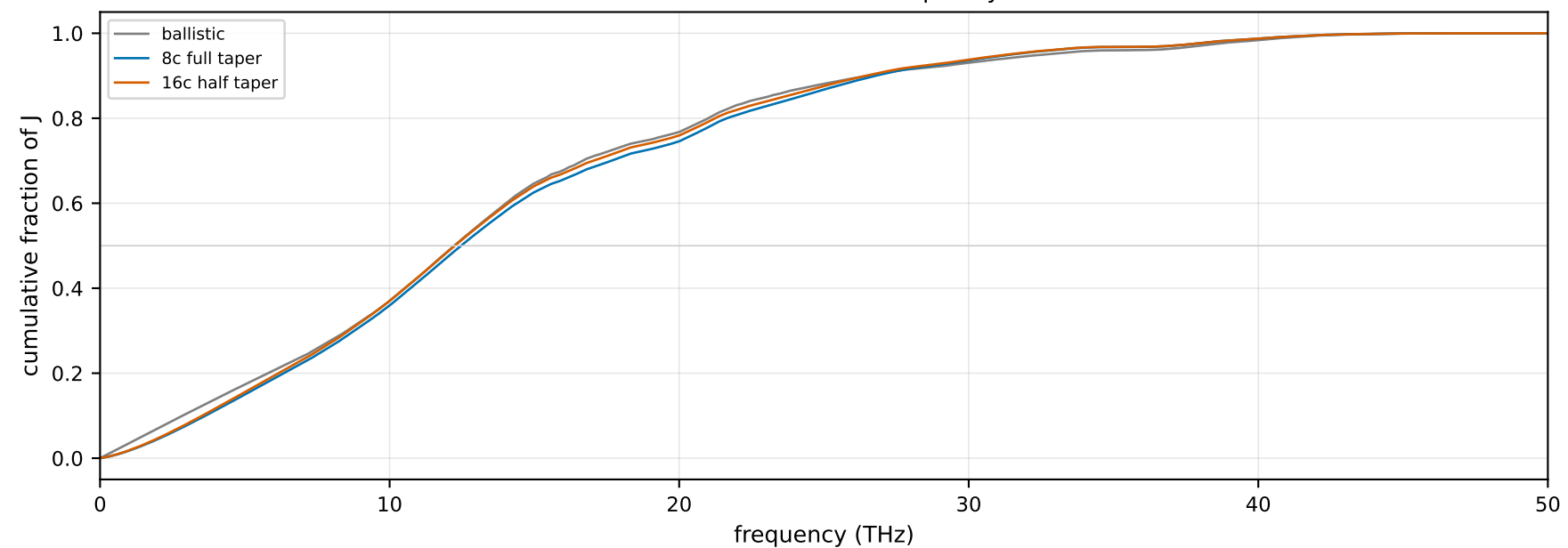
cumulative heat vs frequency
