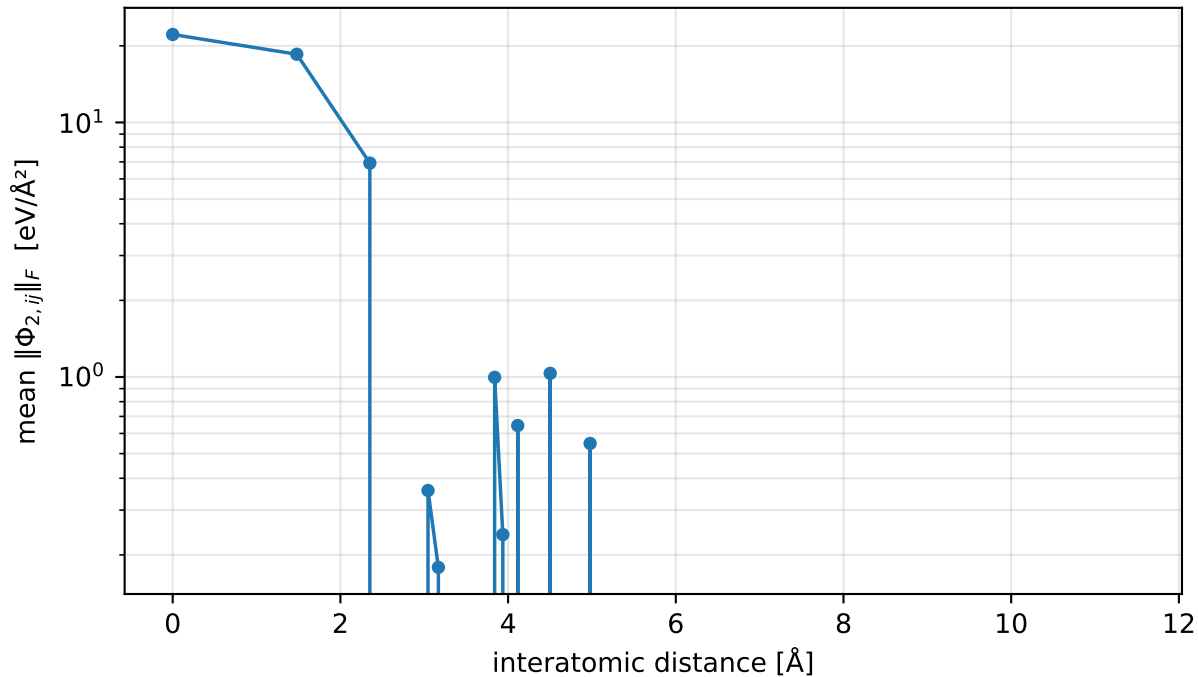
FC2 magnitude vs distance — sinw100_d9a_vasp
