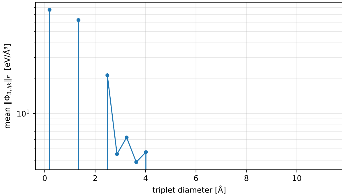
FC3 magnitude vs triplet diameter — sinw100_d9a_vasp
