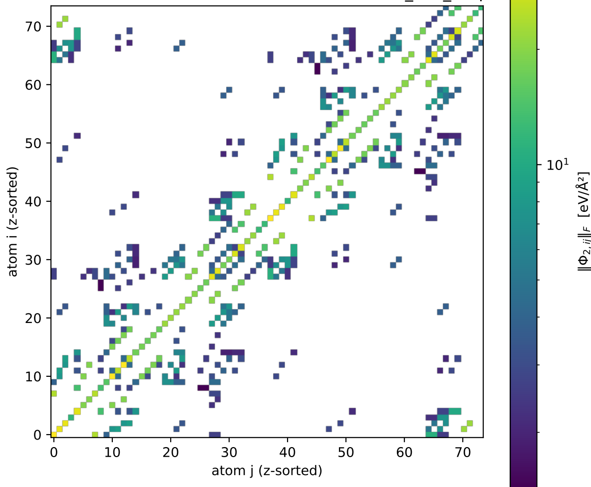
FC2 atomic-block Frobenius norm — sinw100_d9a_vasp
