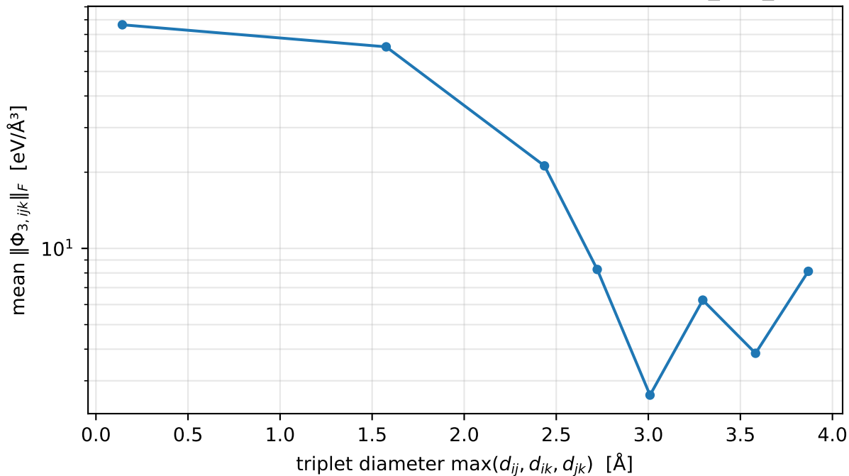
FC3 magnitude decay vs. triplet diameter — sinw100_d9a_vasp
