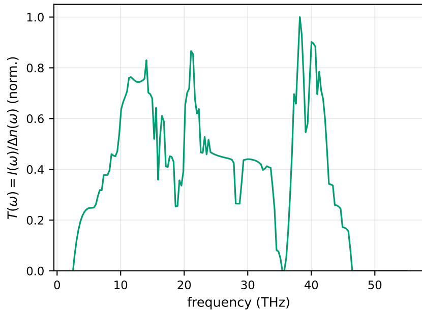
effective transmission ( \omega \geq 2 THz)
