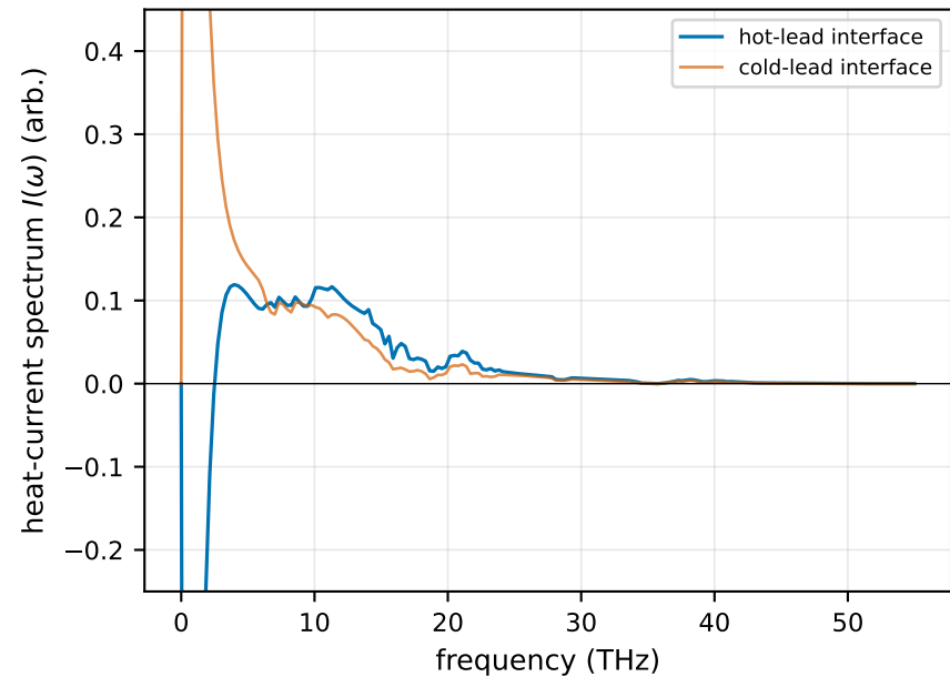
cnt33 \eta = 0 converged: I(\omega)
