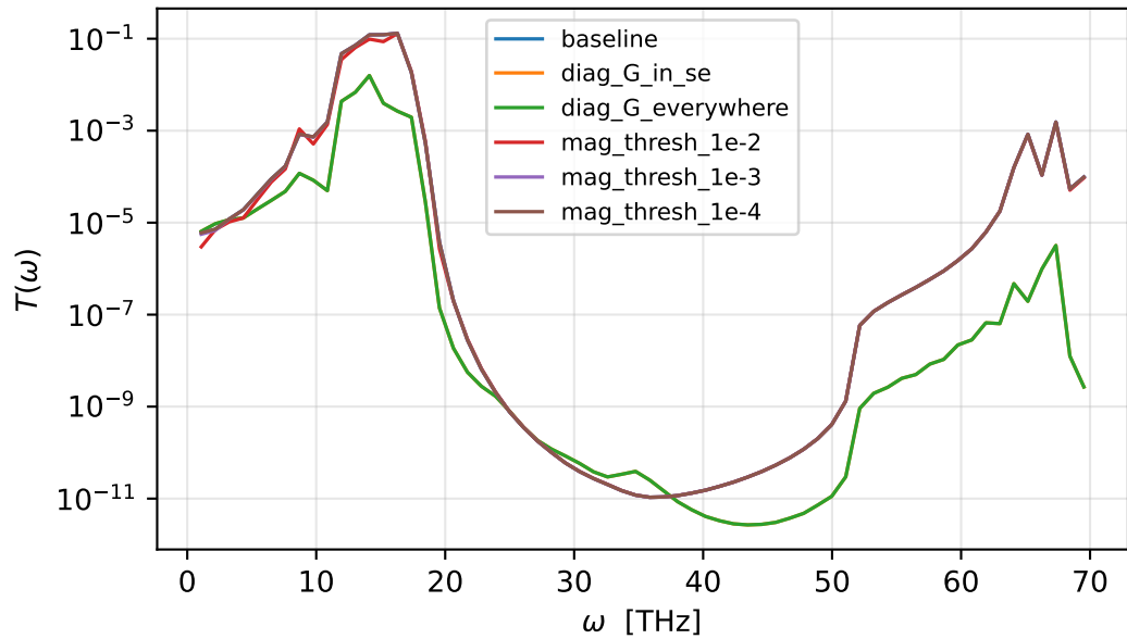
Ballistic transmission — sinw100_d5a_vasp_phonon
