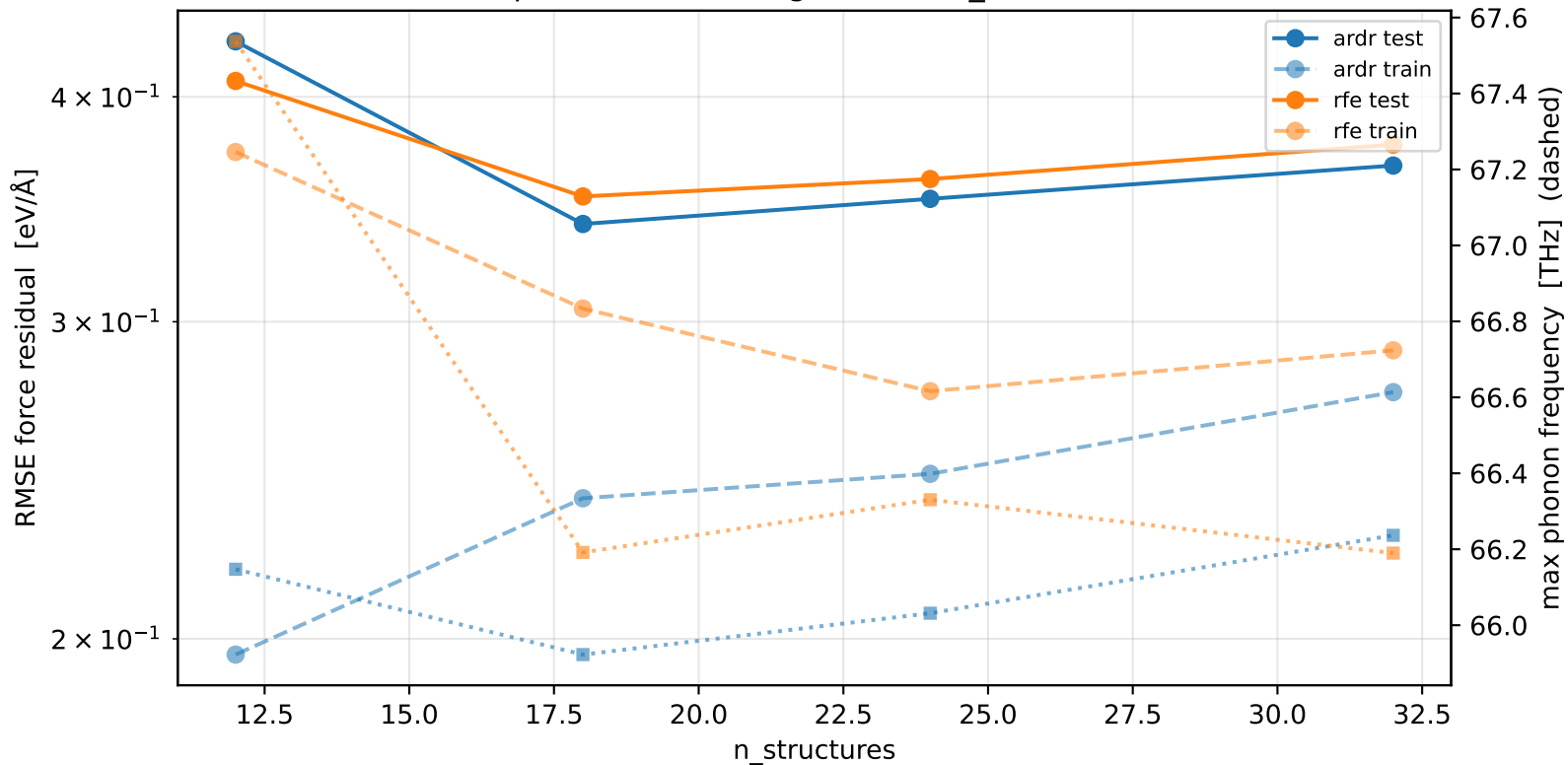
hiphive FC3 convergence vs. n_structures
