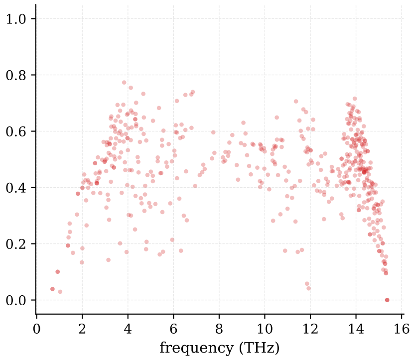
Umklapp fraction of scattering
