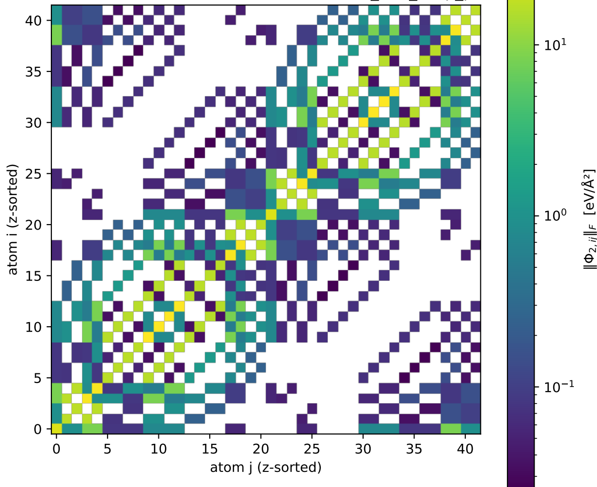
FC2 atomic-block Frobenius norm — sinw100_d5a_vasp_phon
