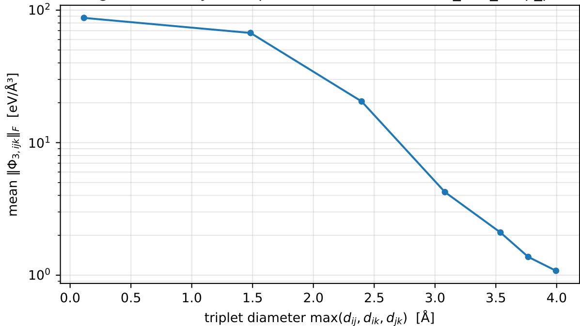
FC3 magnitude decay vs. triplet diameter — sinw100_d5a_vasp_phono
