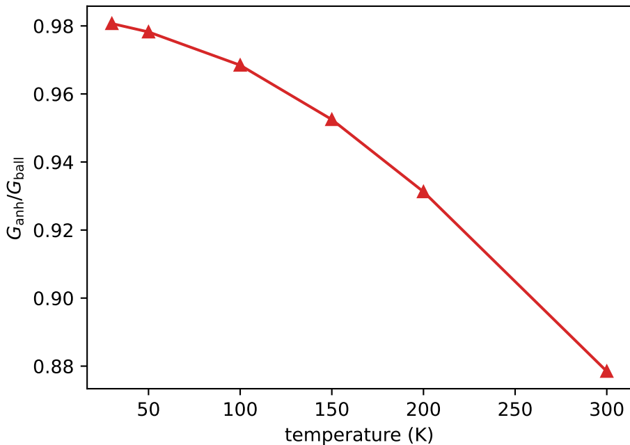
(3,3) CNT: channel freezing as T \rightarrow 0
