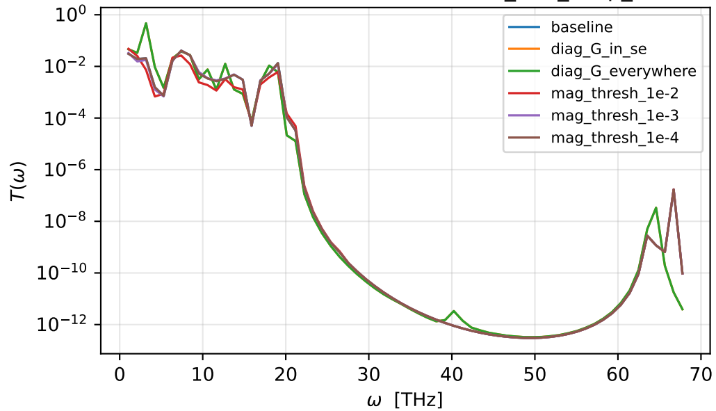
Ballistic transmission — sinw100_d5a_vasp_sc4
