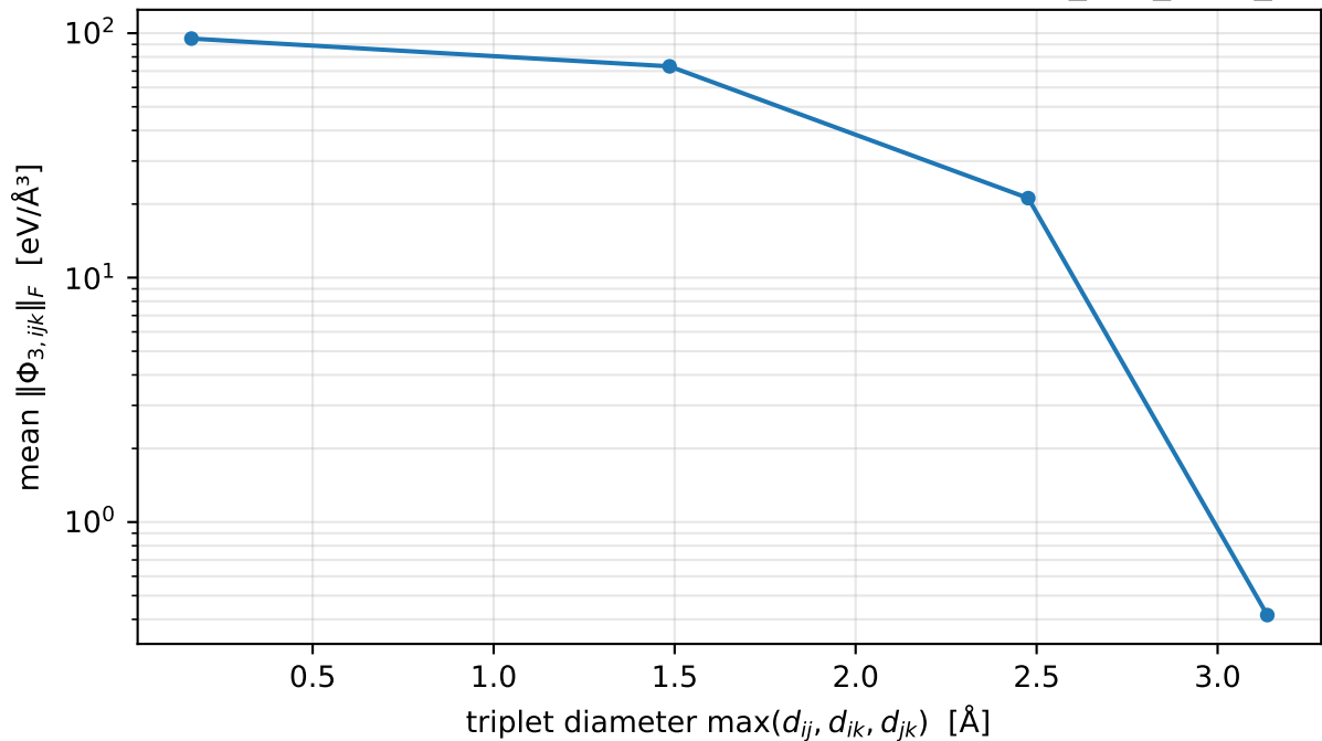
FC3 magnitude decay vs. triplet diameter — sinw100_d5a_vasp_sc4
