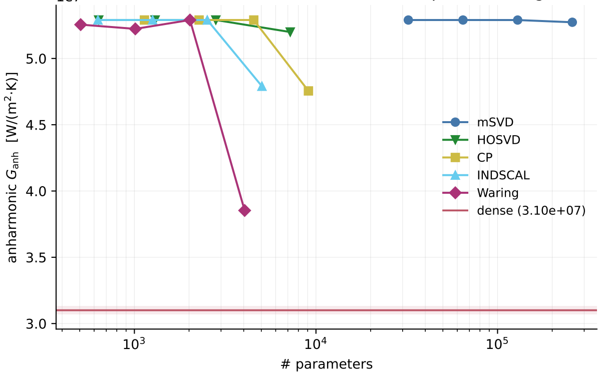
1e7 Anharmonic thermal conductance vs. compression budget
