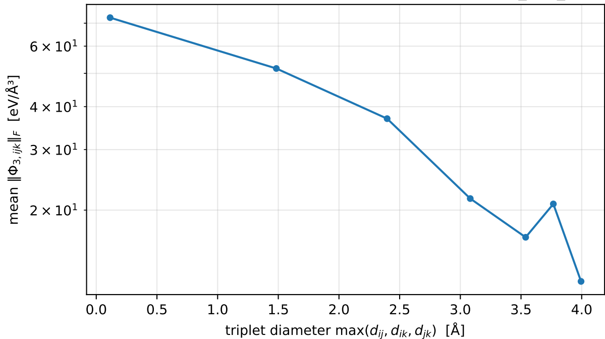
FC3 magnitude decay vs. triplet diameter — sinw100_d5a_vasp
