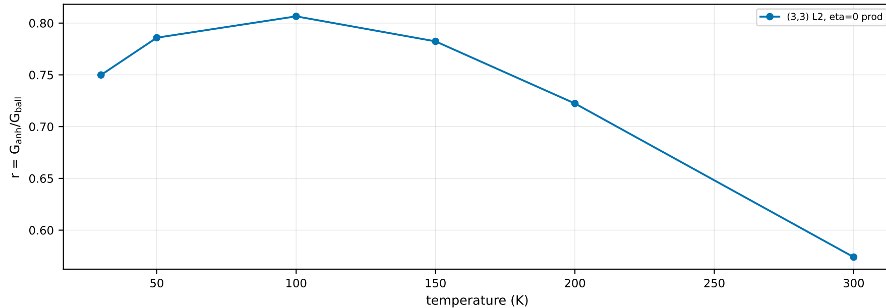
anharmonic suppression vs temperature
