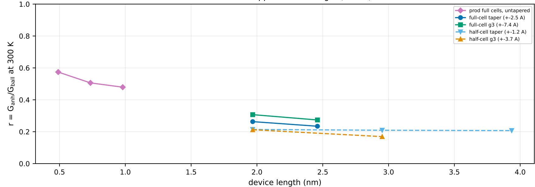
anharmonic suppression vs length ( \eta=0 )
