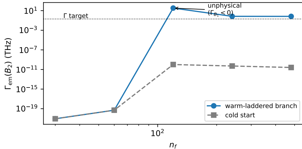
scattering branch vs grid: sustained / unphysical / deleted
