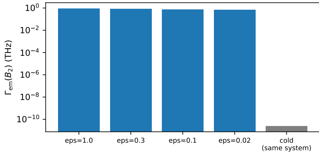
contact-broadening continuation vs cold start (nf=480): two fixed points
