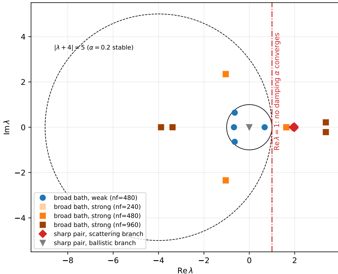
E7: measured Jacobian spectra of the toy SCBA map (top Arnoldi eigenvalues at each fixed point / best iterate)
