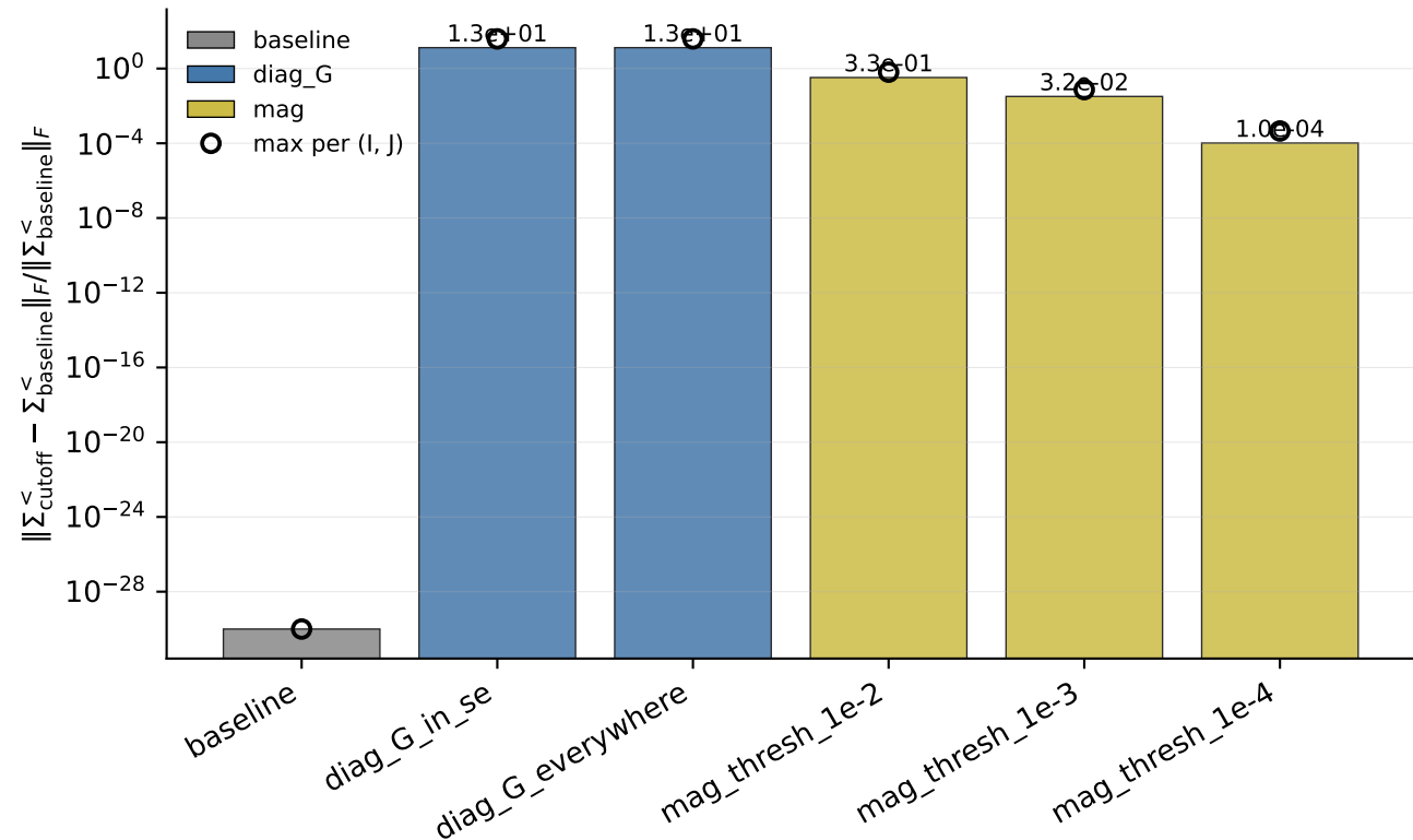
Cutoff sensitivity of phonon-phonon SSE
