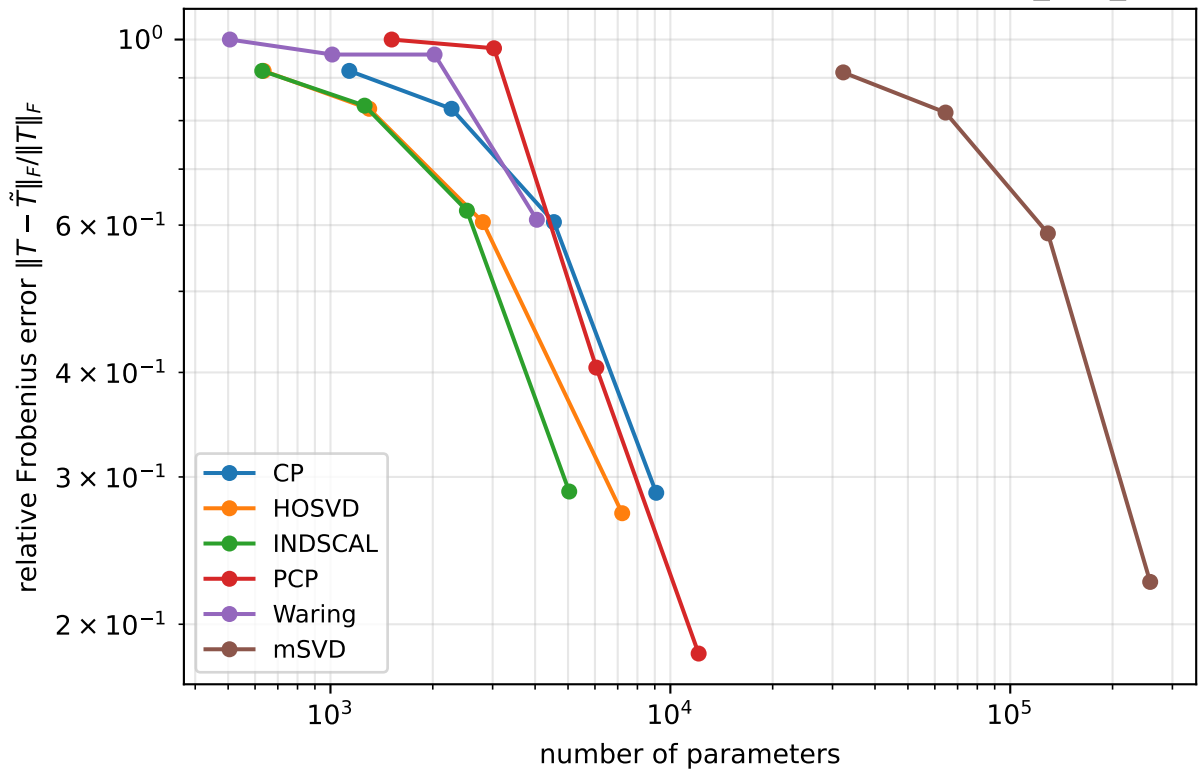
FC3 decomposition: error vs. parameter count — sinw100_d5a_vasp_s
