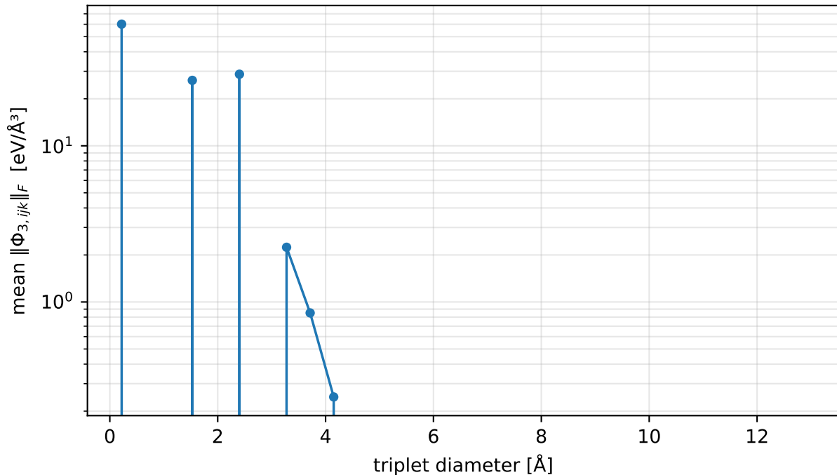
FC3 magnitude vs triplet diameter — sinw100_d5a_vasp_sc4
