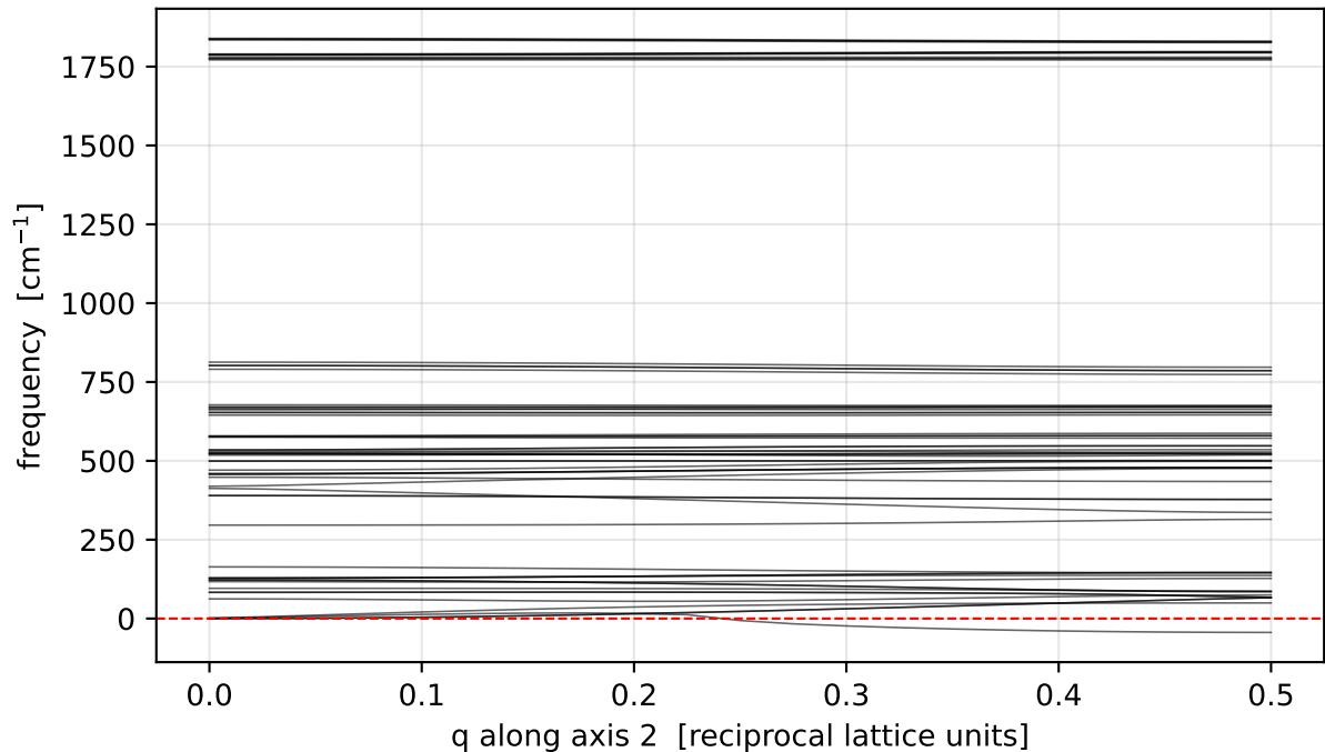
Phonon dispersion (sanity) — sinw100_d5a_vasp_sc4
