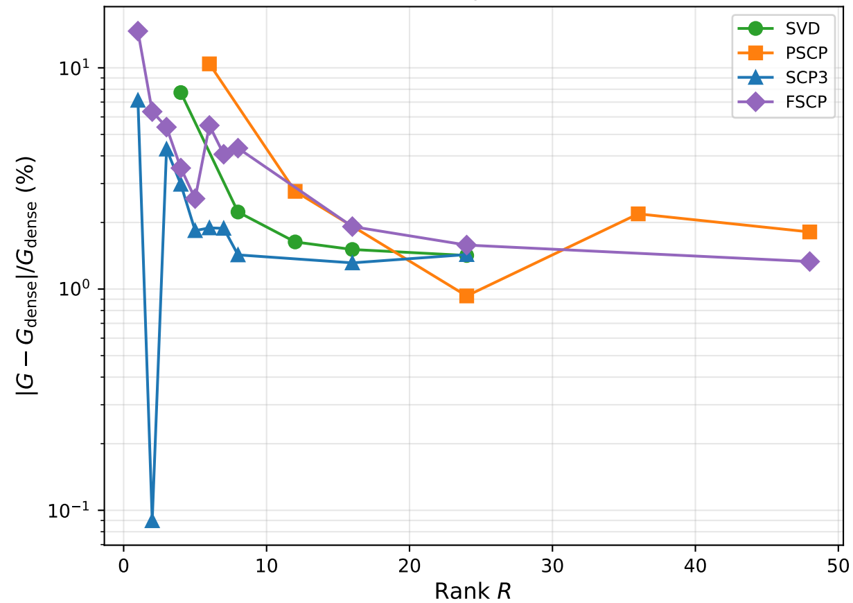
(b) Relative transport error vs rank
