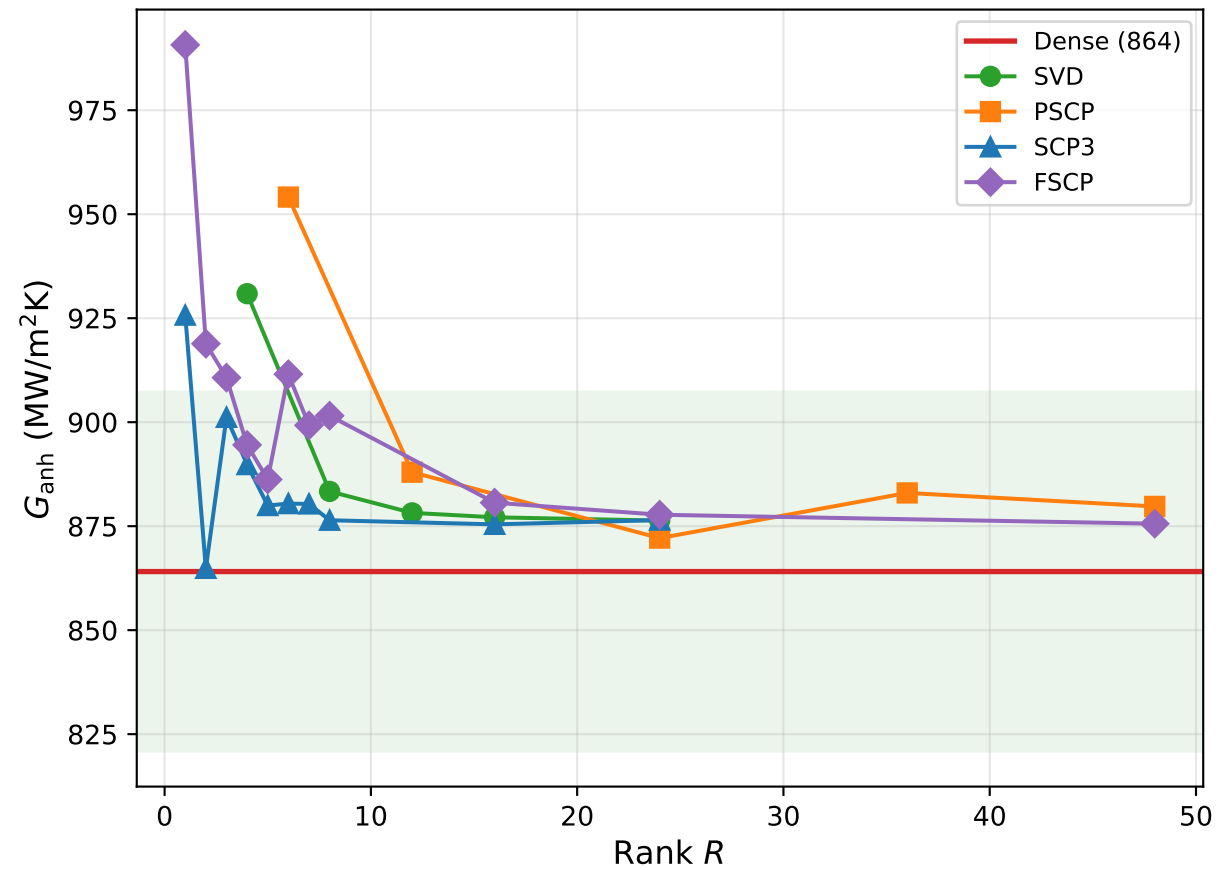
(a) Thermal conductance vs rank
