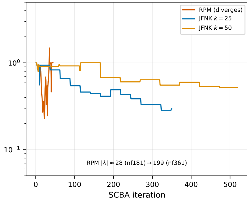
rel \Sigma^R residual
