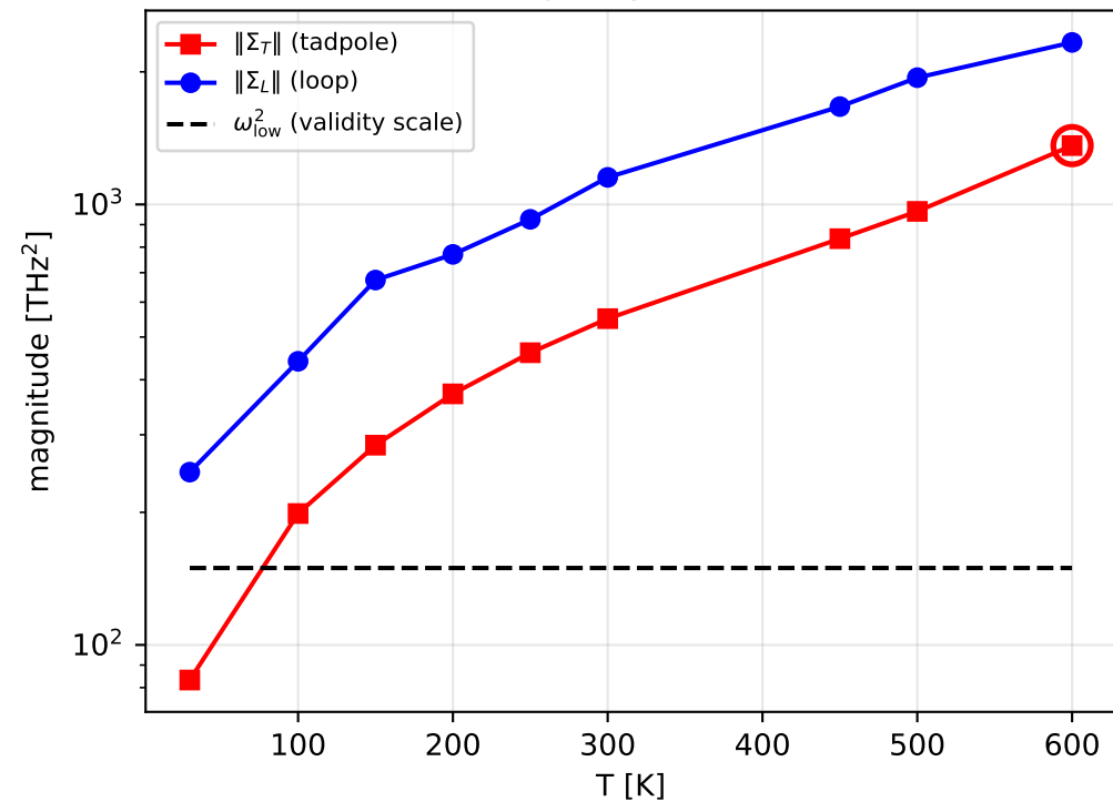
cnt33: tadpole breakdown (circled = imaginary mode / not conv.)
