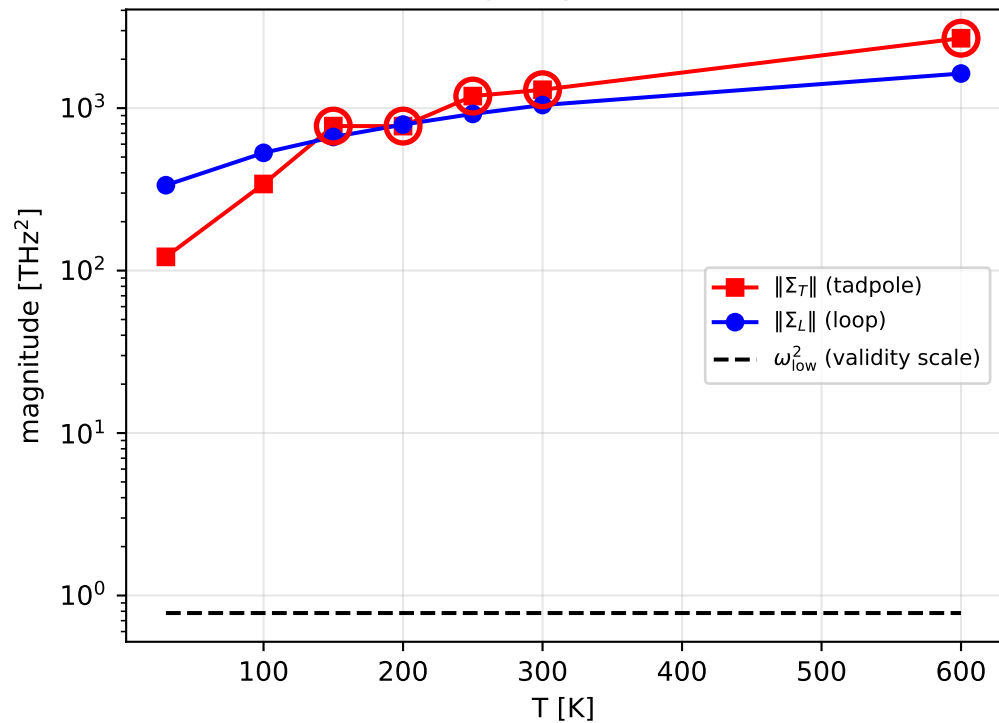
d5a: tadpole breakdown (circled = imaginary mode / not conv.)
