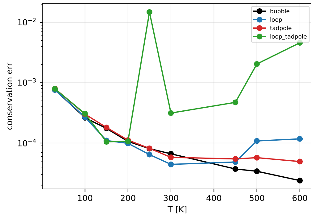
cnt33: heat-flow conservation
