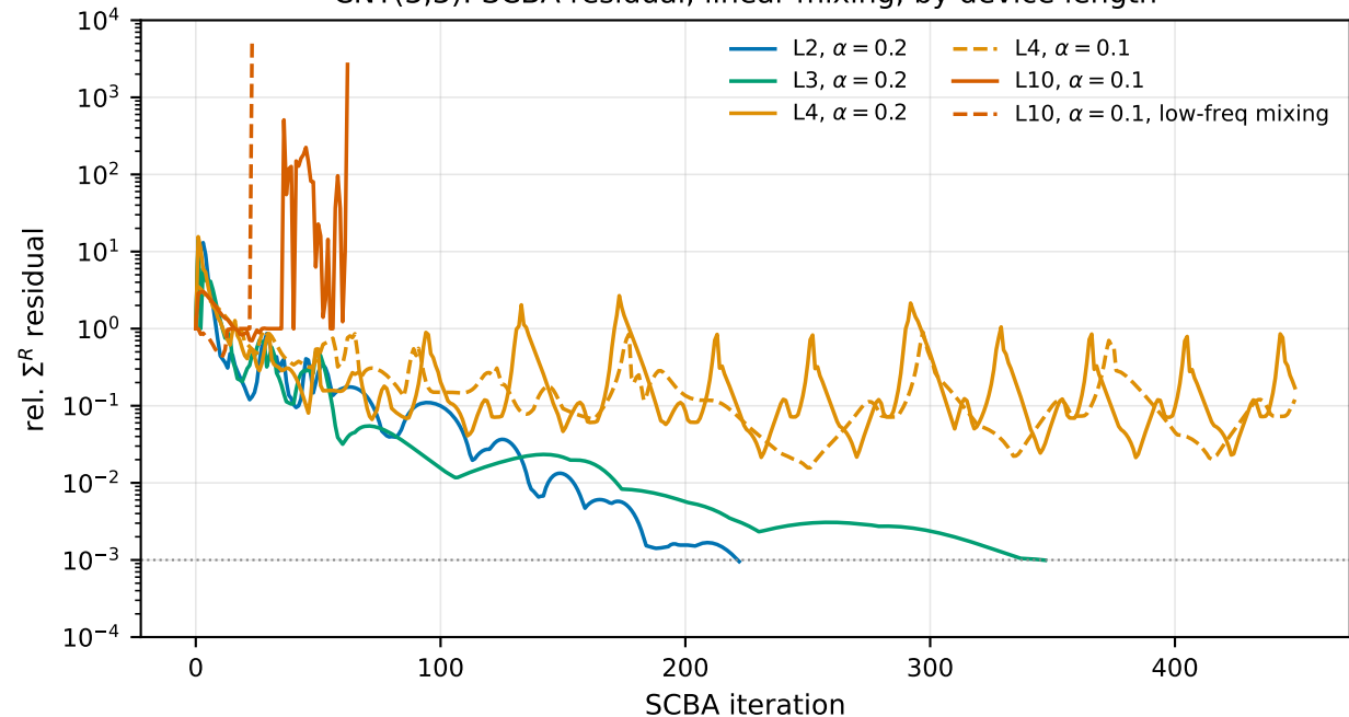
CNT(3,3): SCBA residual, linear mixing, by device length
