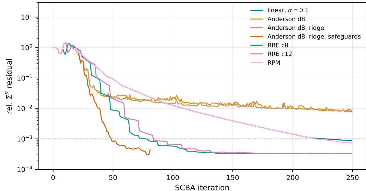
d5a SiNW, \alpha = 0.1 , IR floor: mixing schemes
