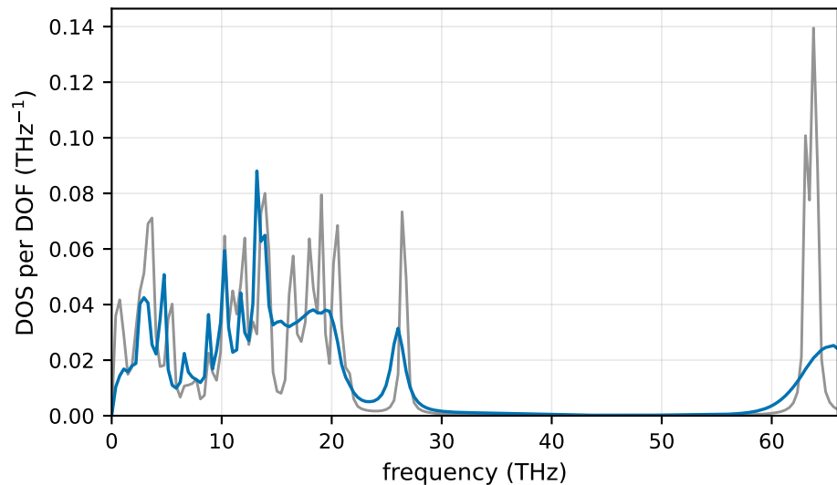
d5a SiNW (sum rule 0.842)
