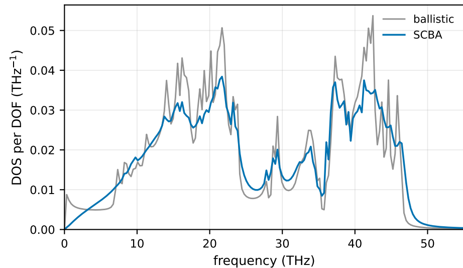
CNT L4* (sum rule 0.961)
